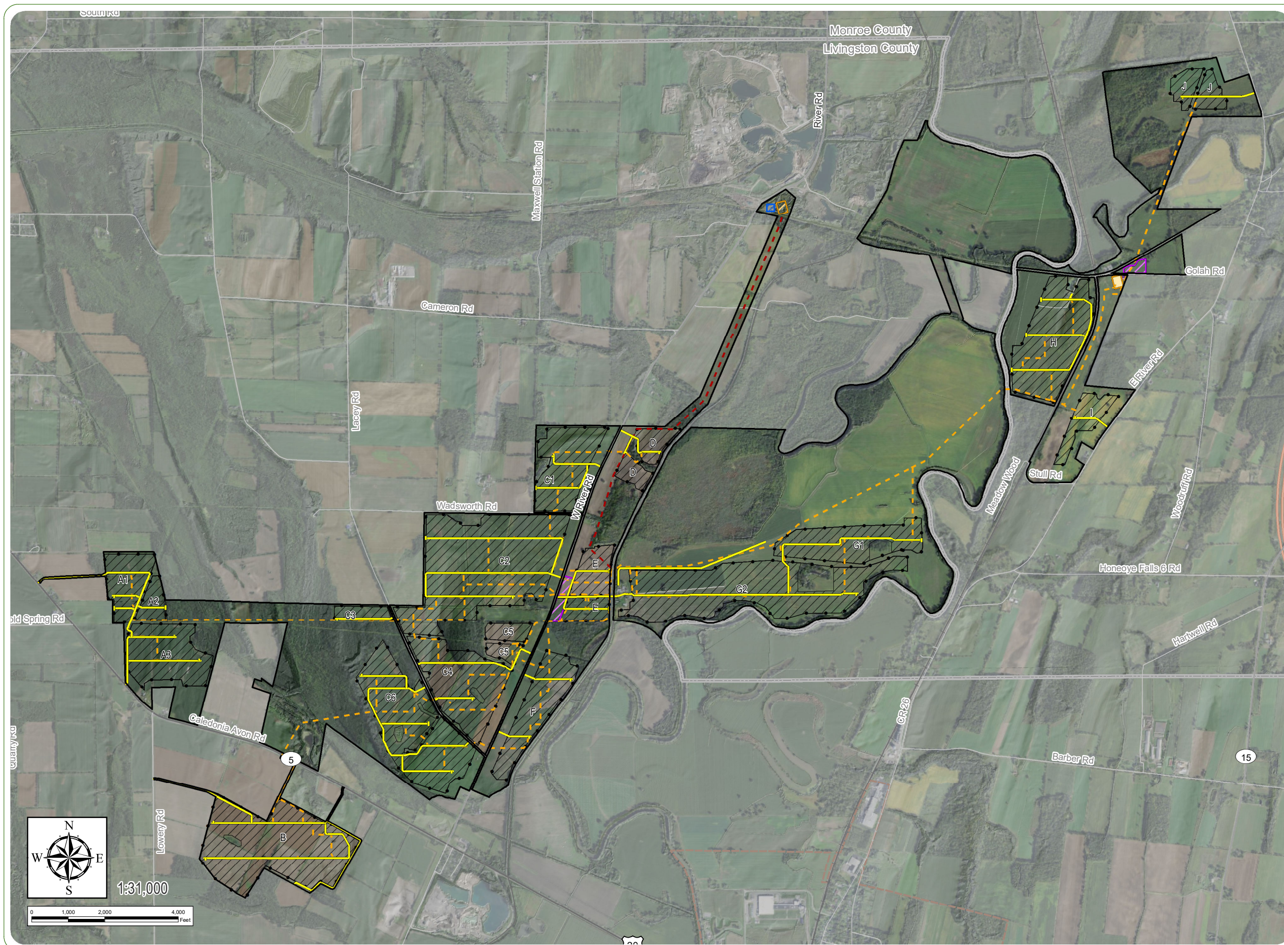
Figure 2-2: Facility Layout
